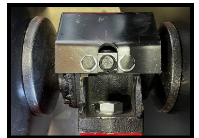
Oil Bath Bearings with Duo-cone seals for easy maintenance
