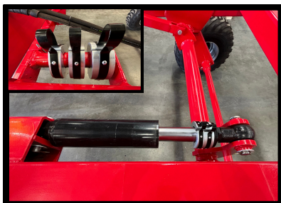
Hydraulic cylinder stopper. Three different stoppers. 1 x 25mm, 1 x 32mm and 1 x 38mm
