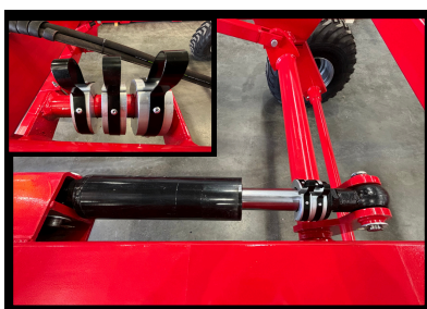
Hydraulic cylinder stoppers 1 x 25mm, 1 x 32mm and 1 x 38mm
